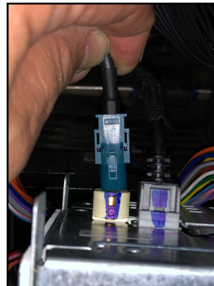
7. Unplug the factory LVDS connector and plug it to the LVDS video board. Plug the LVDS connector from the LVDS video board to the radio.
