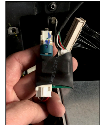
7. Unplug the factory LVDS connector and plug it to the LVDS video board. Plug the LVDS connector from the LVDS video board to the radio.
