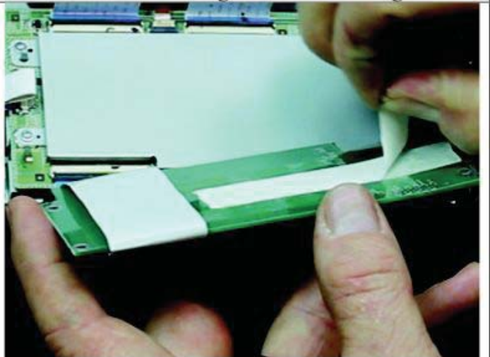
Remove the backing from the double-sided tape of the nav board and secure it to the metal cover below
