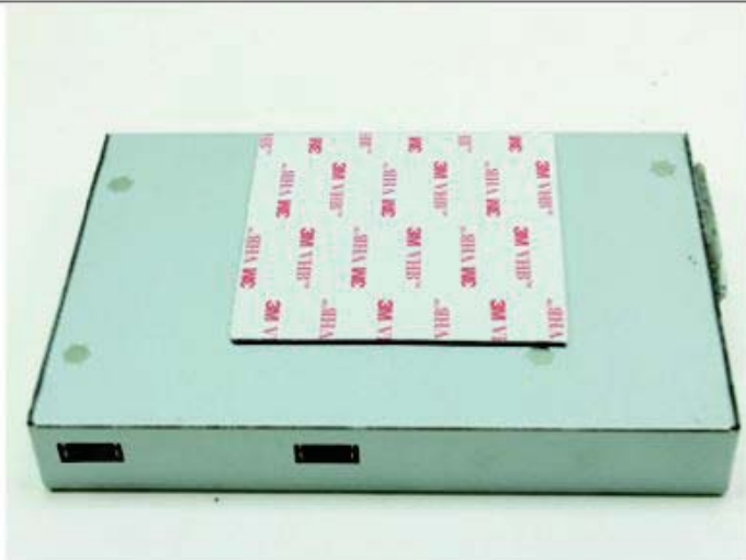
Once clean, press the supplied VHB tape firmly to the bottom side of the navigation module.
