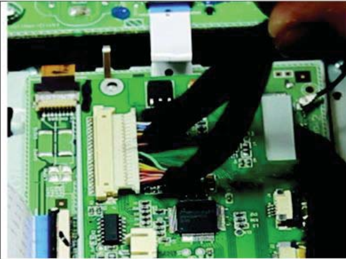
Connect LCD-IN/TP-IN Extension Harness to the navigation interface board.
